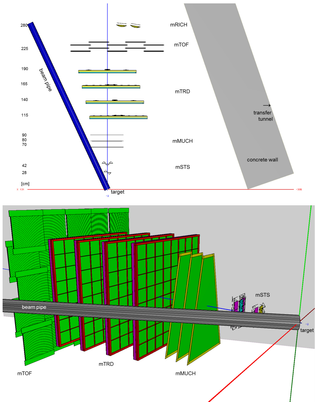
Figure 2: Top view (top panel) and side view (bottom panel) of the mCBM test setup at the HTD cave. The detector stations are aligned at an emission angle of about \Theta_{lab} = 13^\circ (beam pipe side) at y = 0 . The x-, y- and z-axes are respectively plotted as red, green and blue colored lines. The beam pipe is located in the x-z plane, at positive x-coordinates and an angle of 25^\circ with respect to the z-axis. Note, the GEM counters of the mMUCh subsystem are trapezoidal shaped (see lower panel), which is not visible in the top-view projection.
