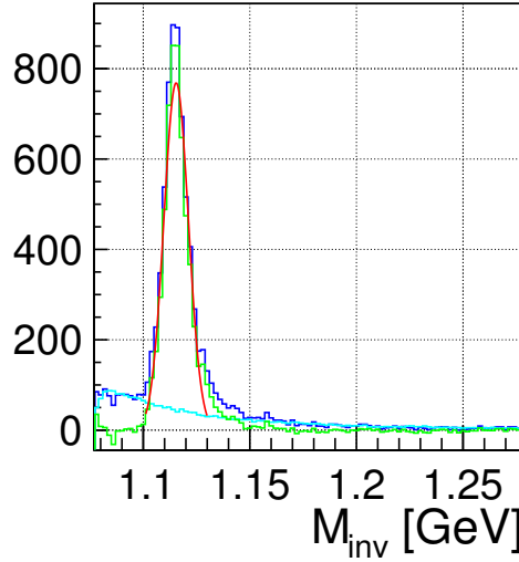
Figure 7: \Lambda -identification in UrQMD events in Ni + Ni collisions at 1.93 AGeV. Invariant mass distributions are shown for pair combinations (combinatorics) within events (dark blue), for pair combinations from mixed events (cyan) and for the subtracted distribution (green). Statistics information is obtained from a gaussian fit to the subtracted distribution (red line) and is summarized in Table 5.
