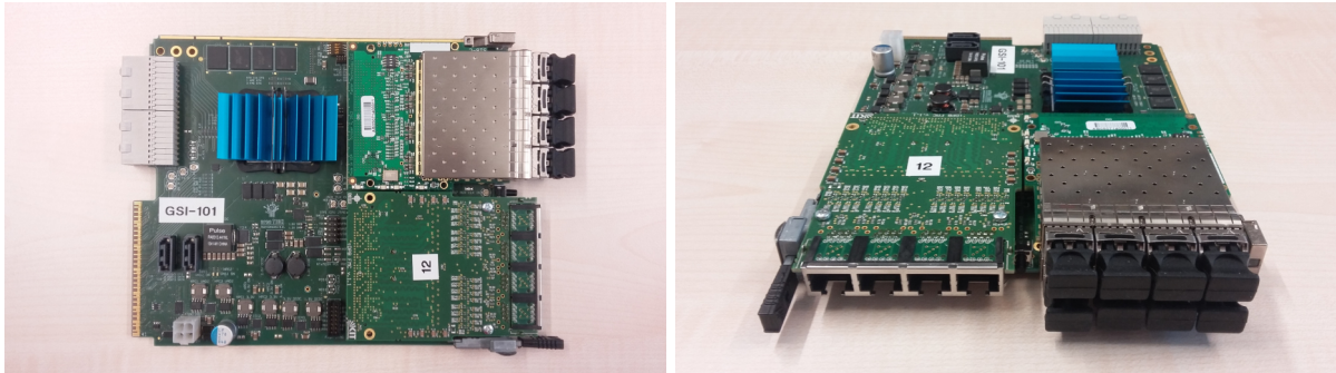
Figure 29: AMC FMC Carrier Kintex (AFCK) board, a Xilinx Kintex-7 FPGA board in AMC form factor equipped with a FM-S18 FMC and a tDPB FMC. An AFCK with this configuration can be used to interface 6x incoming GBT links at 4.48 Gbit/s to 1x outgoing FLIM link.
